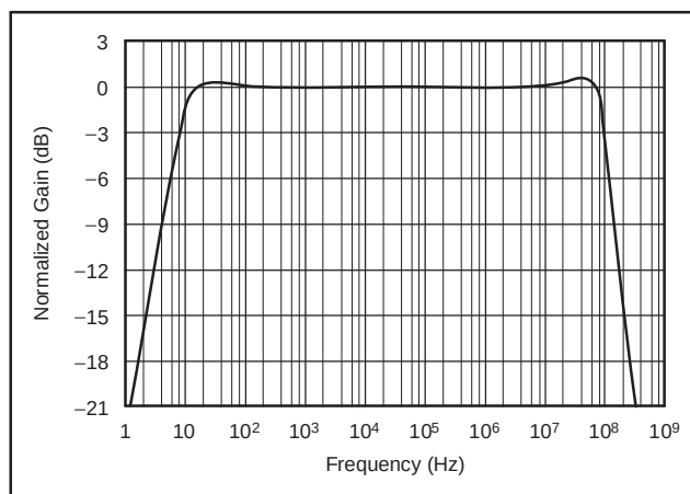
Figure 75. Video Line Driver Response to Matched Load
