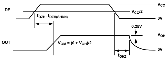
Figure 10. Driver Enable and Disable Times ( t_{DZH} , t_{DZH(SHDN)} , t_{DZH} )
