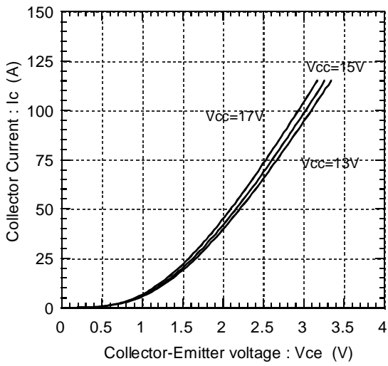
Collector current vs. Collector-Emitter voltage (typ.) Tj=125°C(Chip)
