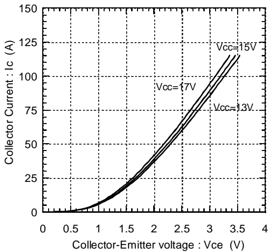
Collector current vs. Collector-Emitter voltage (typ.) Tj=125°C(Terminal)
