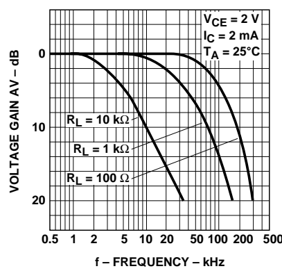
Figure 11. Frequency response.
