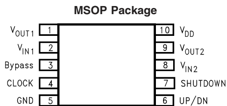
Top View Order Number LM4811MM See NS Package Number MUB10A
