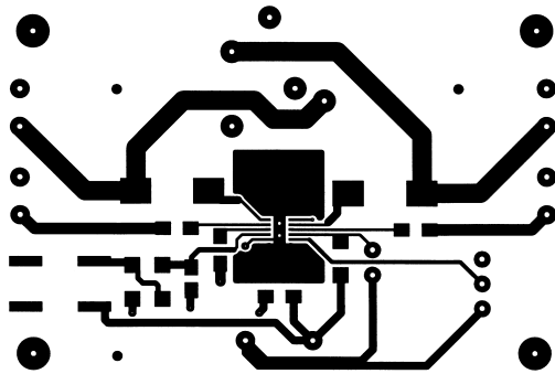
FIGURE 8. Recommended LD PC Board Layout: TOP Top Layer
