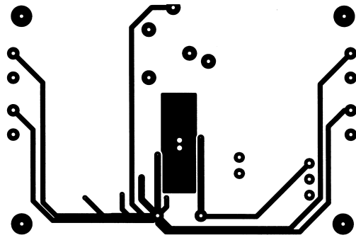
FIGURE 9. Recommended LD PC Board Layout: Bottom Layer
