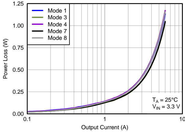
Figure 15. Power Loss
