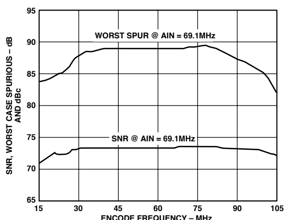
TPC 18. SNR, Worst Spurious vs. Encode @ 69.1 MHz
