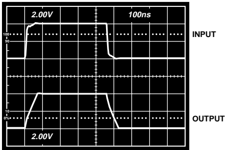
Figure 10. Noninverting Large Signal Pulse Response, R_L = 500 \Omega , V_S = \pm 12 V , G = 1 , R_F = 0
