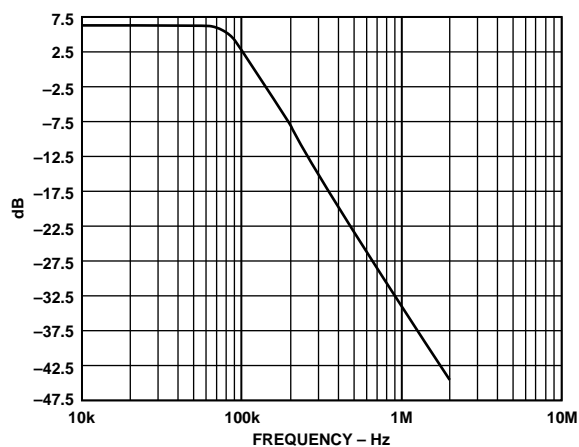
Figure 39. Frequency Response of Sallen-Key Filter
