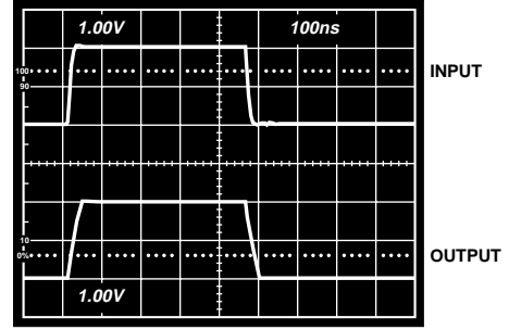
Figure 13. Noninverting Large Signal Pulse Response, R_L = 500 \Omega , V_S = \pm 2.5 V , G = 1 , R_F = 0
