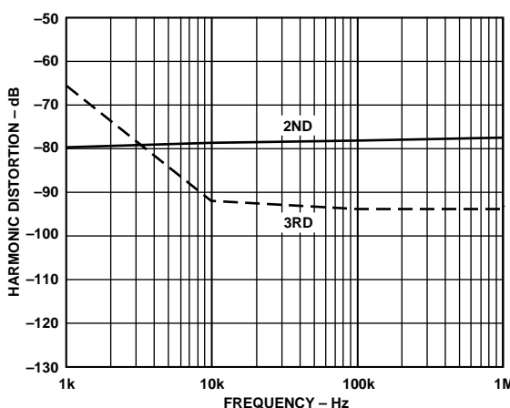
Figure 19. Distortion vs. Frequency, V_S = \pm 2.5\text{ V} , R_L = 500\ \Omega , R_F = 715\ \Omega , V_{OUT} = 2\text{ V p-p} , Gain = 1
