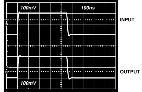
Figure 12. Noninverting Small Signal Pulse Response, R_L = 500 \Omega , V_S = \pm 2.5 V , G = 1 , R_F = 0
