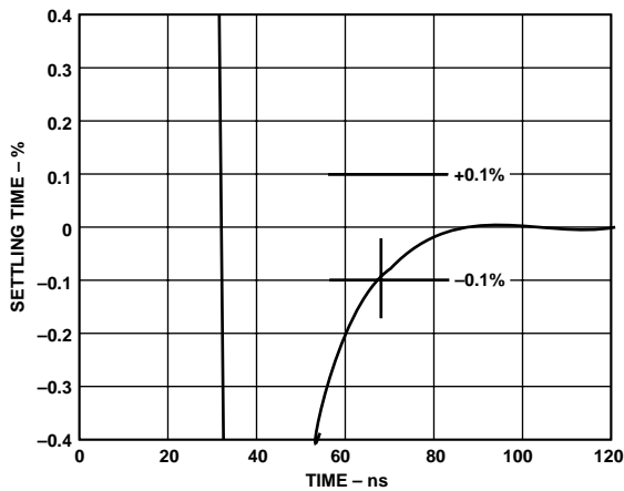
Figure 11. Settling Time to 0.1%, V_S = \pm 12 V , Step Size = 2 V p-p, G = 2 , R_L = 500 \Omega
