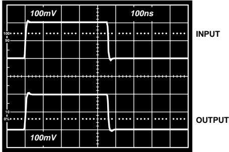
Figure 9. Noninverting Small Signal Pulse Response, R_L = 500 \Omega , V_S = \pm 12 V , G = 1 , R_F = 0
