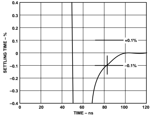
Figure 14. Settling Time to 0.1%, V_S = \pm 2.5 V , Step Size = 2 V p-p, G = 2 , R_L = 500 \Omega
