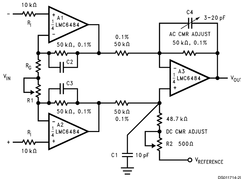
FIGURE 15. Low Power 3 Op-Amp Instrumentation Amplifier
