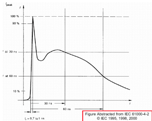
Figure 7. I_{\text{peak}} = f(t) /IEC61000-4-2
